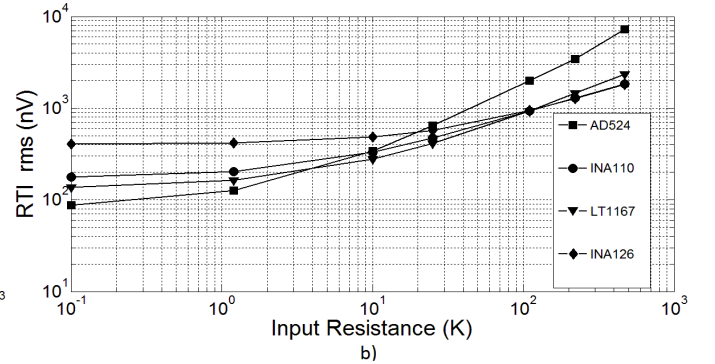
Fig. 9. Noise comparison of the four instrumentation amplifiers: a) theoretical, b) experimental.
