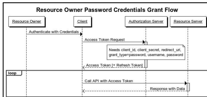
Figura 10: Resource Owner Password Credentials Grant Flow.
