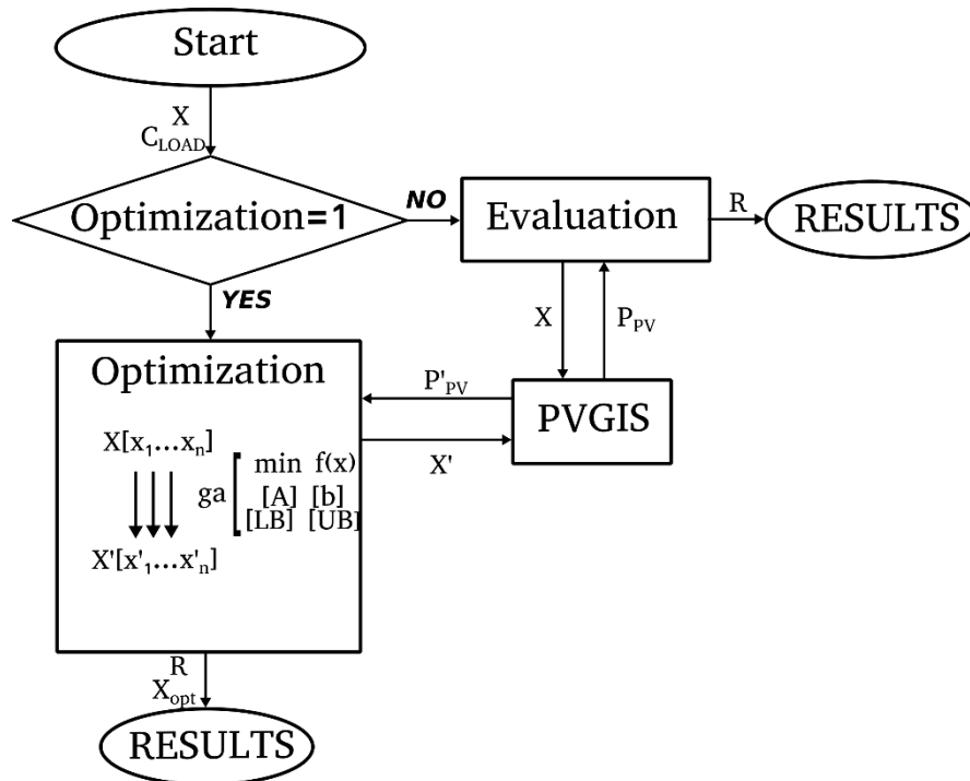
Fig. 4: Algorithm flowchart.
