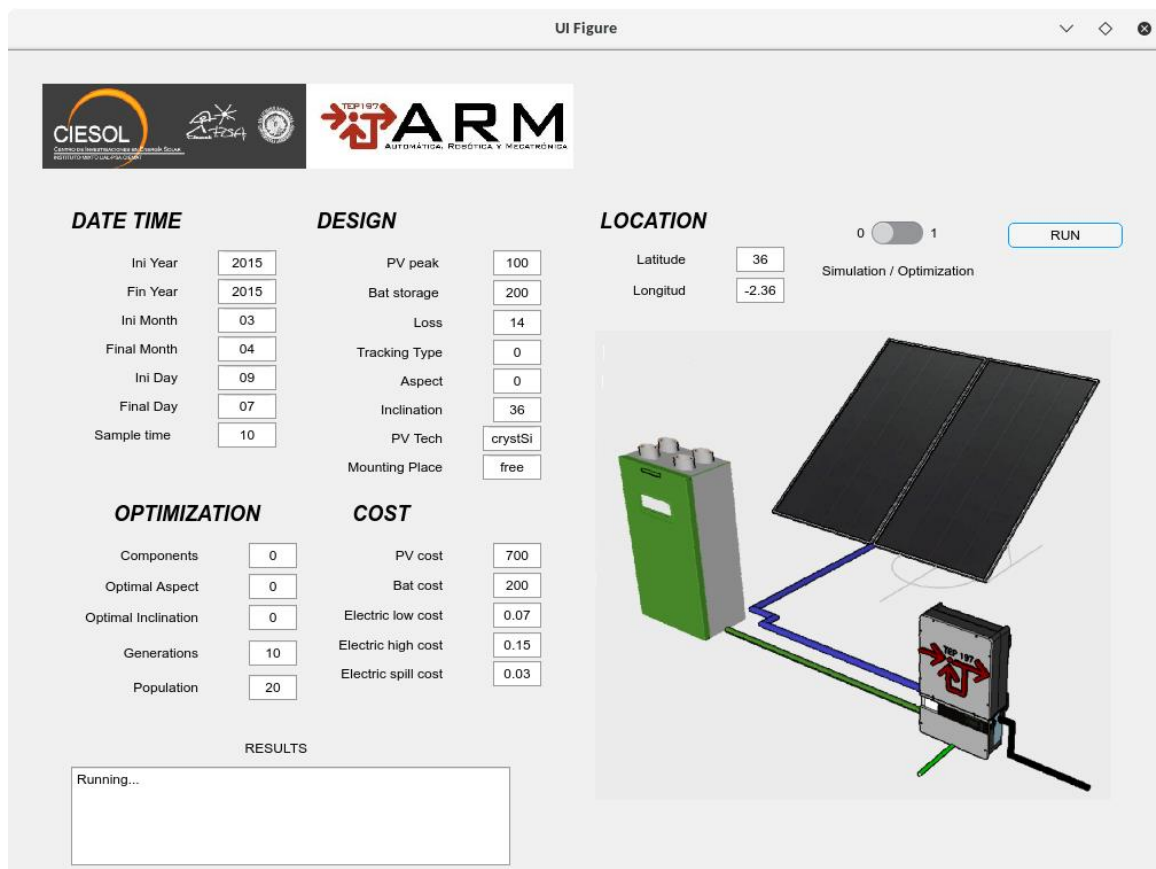
Fig. 5: GUI layout.
