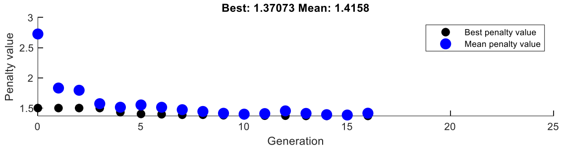
Fig. 7: Optimization process.
