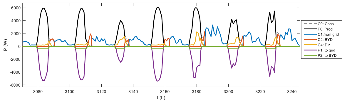
Fig. 9: Winter solstice week.
