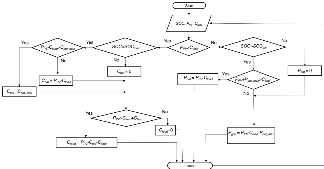
Fig. 3: Flowchart describing the power exchange rules in a typical household energy storage system.
