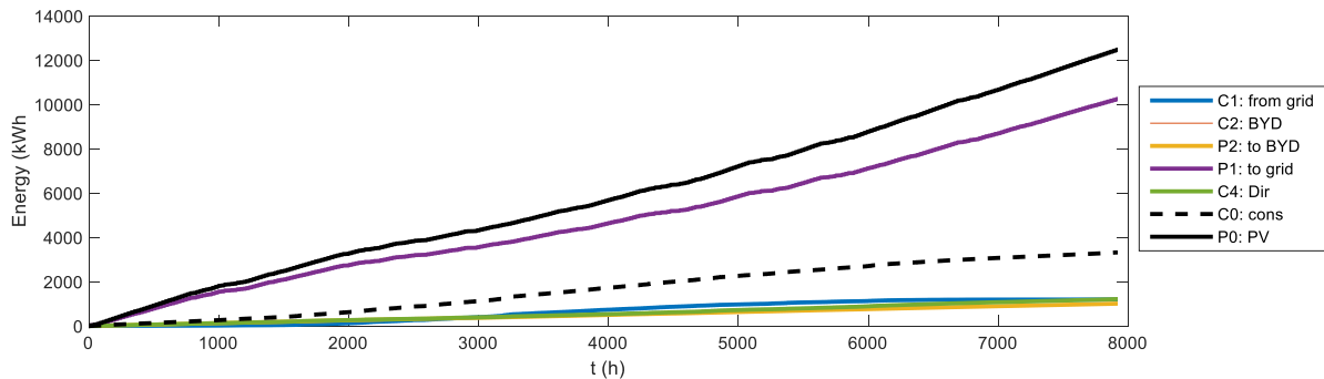
Fig. 8: Total system behavior.
