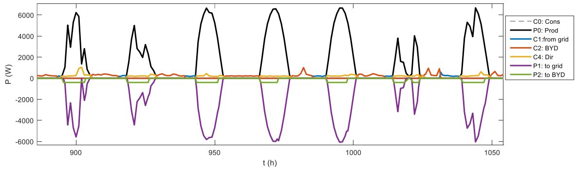
Fig. 8: Autumn equinox week.
