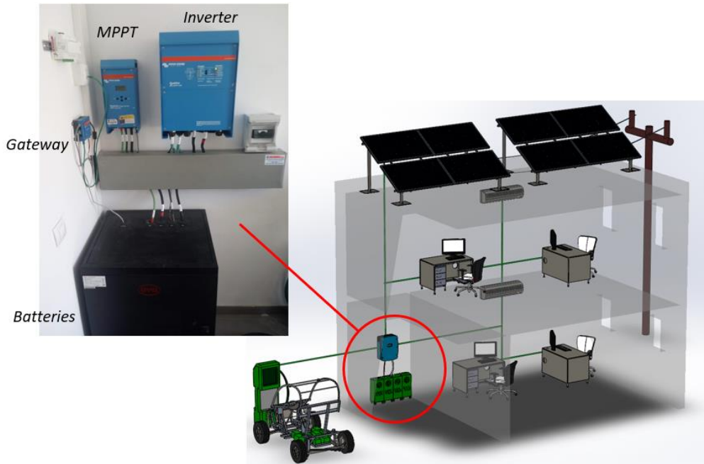
Fig. 2: A microgrid for a small office building. On the left side, it is represented the real equipment, whose characteristics can fit to an installation as the one depicted on the right side.
