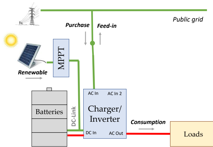
Fig. 1: DC-Link configured PV-Battery system
