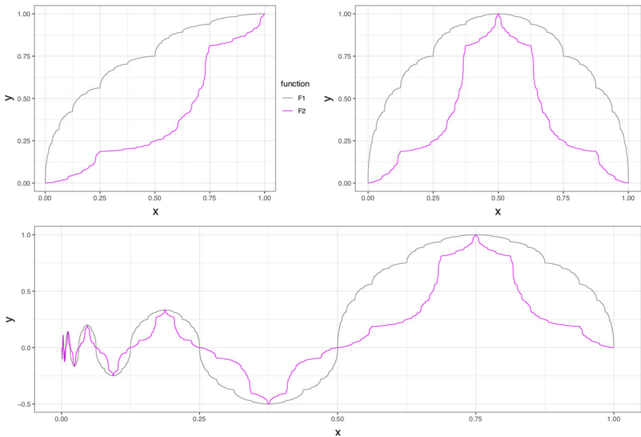
Fig. 1 Two choices for the singular function F (upper left panel), the functions f according to Eq. 2.2 (upper right panel), and the resulting functions \Phi_f(\mathbf{s}) for \mathbf{s} = (s_1, s_2, s_3, \dots) with s_i = \frac{1}{i}(-1)^{i+1} (lower panel). Both functions F were constructed via fractal interpolation as discussed in [26] (see, also, [13])
