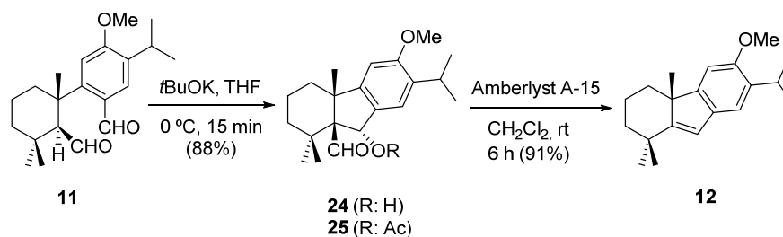
Scheme 4. Synthesis of compound 12 from dialdehyde 11 , via aldol 24 .
