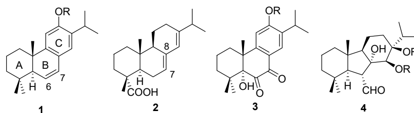
Figure 2. Abietane-type compounds ( 1–2 ) and their synthetic derivatives ( 3–4 ).
