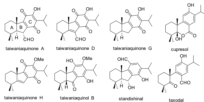
Figure 1. Representative taiwaniaquinoids and related metabolites.
