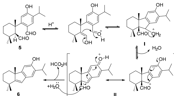
Scheme 3. Mechanism for the transformation of dialdehyde 5 into phenol 6 .
