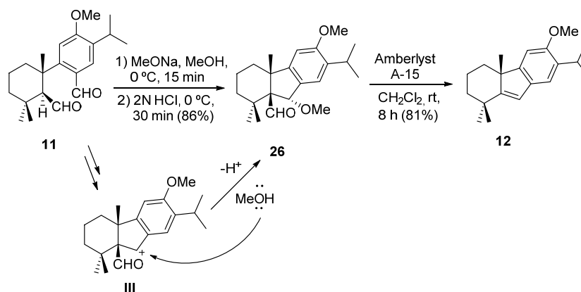
Scheme 5. Synthesis of compound 12 from dialdehyde 11 , via O -methyl aldol 26 .
