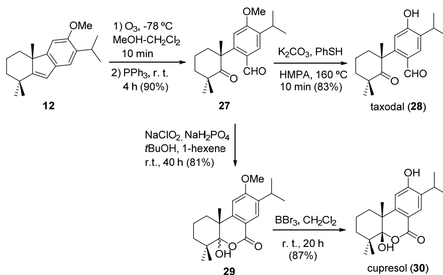
Scheme 7. Synthesis of taxodal (28) and cupresol (30).
