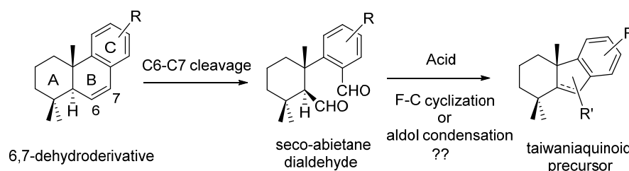
Scheme 1. Abietane B ring contraction via C6–C7 cleavage.
