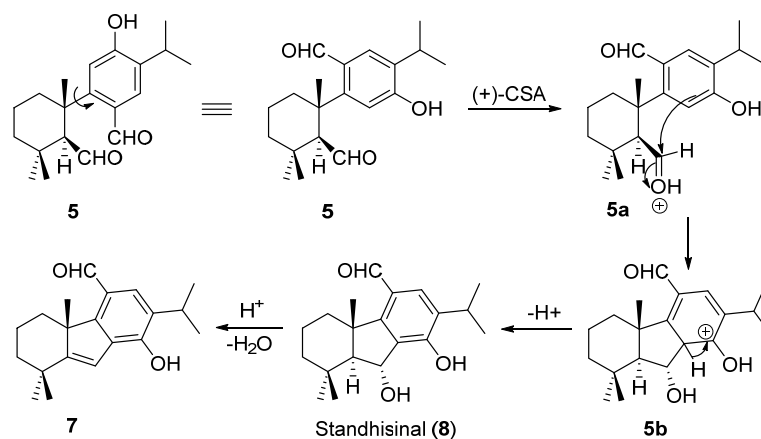
Scheme 2. Mechanism for the transformation of dialdehyde 5 into standishinal ( 8 ) and compound 7 .
