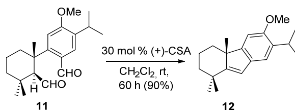
Scheme 6. Cyclization of dialdehyde 11 using a substoichiometric quantity of acid.
