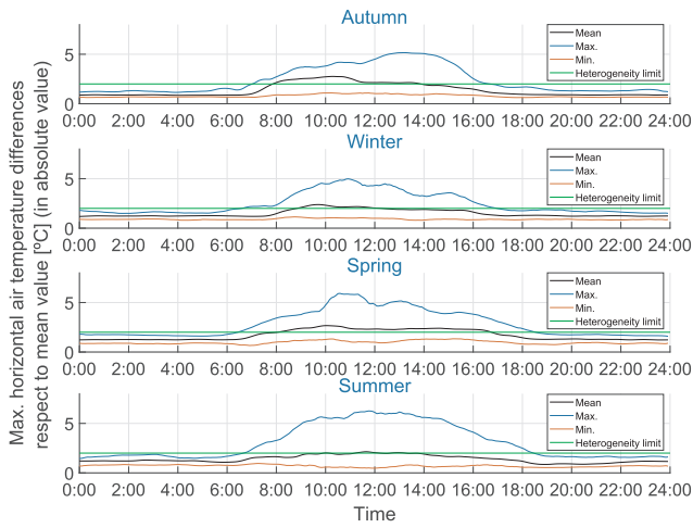
Fig. 15. Maximum horizontal air temperature differences respect to mean value, in absolute value.
