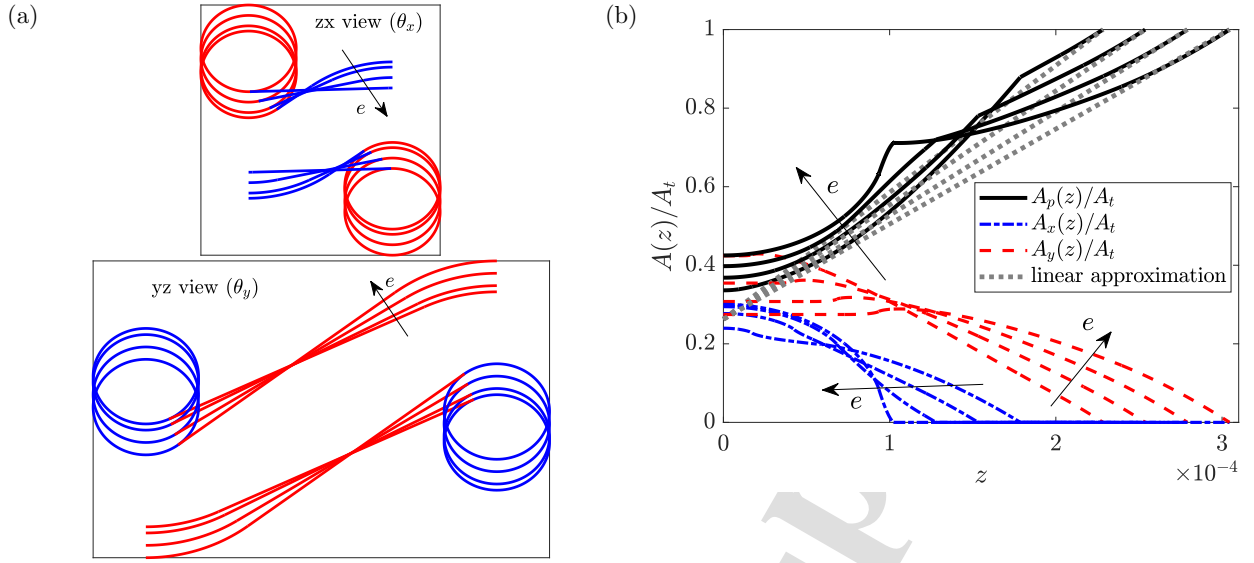
Figure 11: Effect of increasing the thickness of the screen e with the OAT method on a) the wire screen geometry, and b) the local area of the pore A_p/A_t and area occupied by each thread ( A_x for x-thread and A_y for y-thread) when intersected by the plane. Arrows indicate the trend of the plots when the thickness is increased. All units are in meters.
