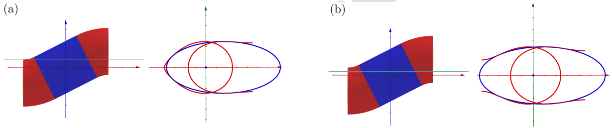
Figure 5: Full cross-sections involving both the upper and bottom toroid portions. a) Upper toroid portion delimited by the vertical symmetry axis and bottom toroid portion delimited by the inner hole. b) Both upper and bottom toroid portions delimited by their vertical symmetry axes.
