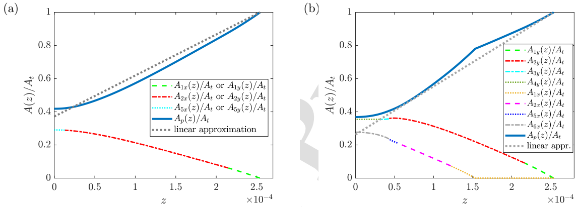
Figure 8: Plots of the analytical estimation of the area of the pore with z and cross-sectional areas of the threads/wires A_{S_{D_m x}}(z) and A_{S_{D_m y}}(z) from the intersection by the plane for each Stretch S_{D_m} present. The dashed lines represent the linear approximation by Wang et al. [66]. The results are made dimensionless with the total projected area A_t and shown for: a) Fully symmetric mesh ( \rho_t = 40 \times 40 in [66]), and b) Notably asymmetric mesh ( N_{WS} = 17 in [14]). All units are in meters.
