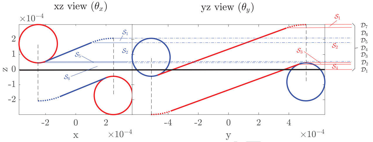
Figure 6: Stretches for an specific mesh with Configuration 2 ( N_{WS} = 11 ). Warp threads are shown in red, and weft in blue. It can be observed all the stretches \mathcal{S} that lead to the definition of the seven Discretisations \mathcal{D} . Both xz and yz views are placed together for better comprehensive interpretation of the definition of the Discretisations. Stretches from the xz view are extended by means of dashed lines to overlap all the stretches at the right hand-side for better identification of Discretisations. The horizontal black thick line represents z = 0 , as only one half is analysed due to symmetry. All units are in meters.
