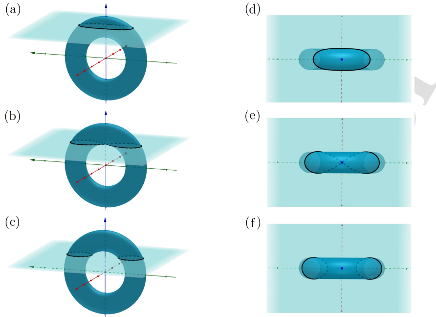
Figure A.12: Different cross-sections of a torus generated by revolution around the x -axis. The left column illustrates the isometric views of the a) Type 1 cross-section, b) Type 2 cross-section, and c) Type 3 cross-section; whereas the right column of plots illustrates the top views of the d) Type 1 cross-section, e) Type 2 cross-section, and f) Type 3 cross-section.
