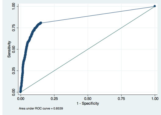
Fig. 2. ROC curves for univariate Probit models
