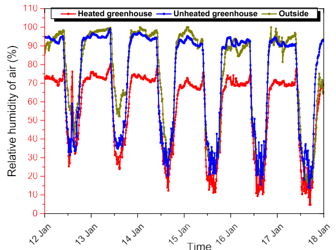
Fig. 9. Evolution of humidity relative in heated/unheated greenhouse and ambient humidity from 12th to 17th, 2020.
