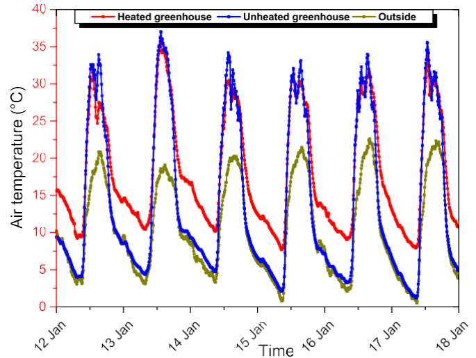
Fig. 8. Evolution of air temperature inside the heated greenhouse, unheated one and outside from 12th to 17th January 2020.
