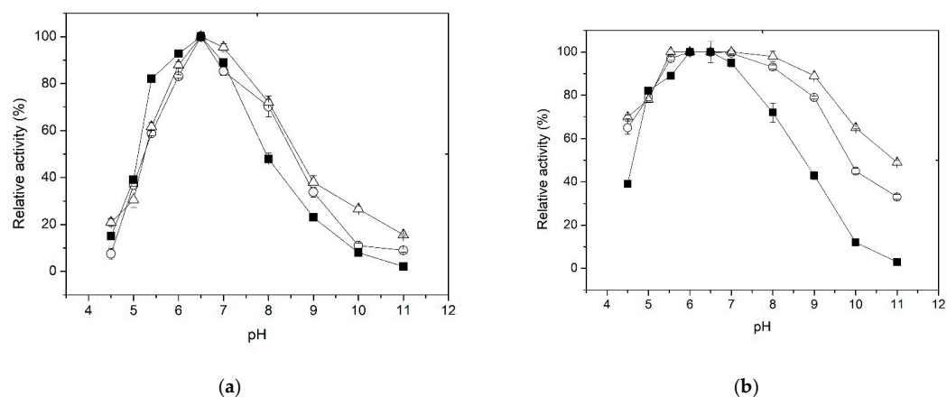
Figure 4. Effect of pH on the \beta -xylosidase activity (a) and stability (b) of free (■) and immobilized enzymes on chitosan by entrapment (○) and covalent bonds (△).
