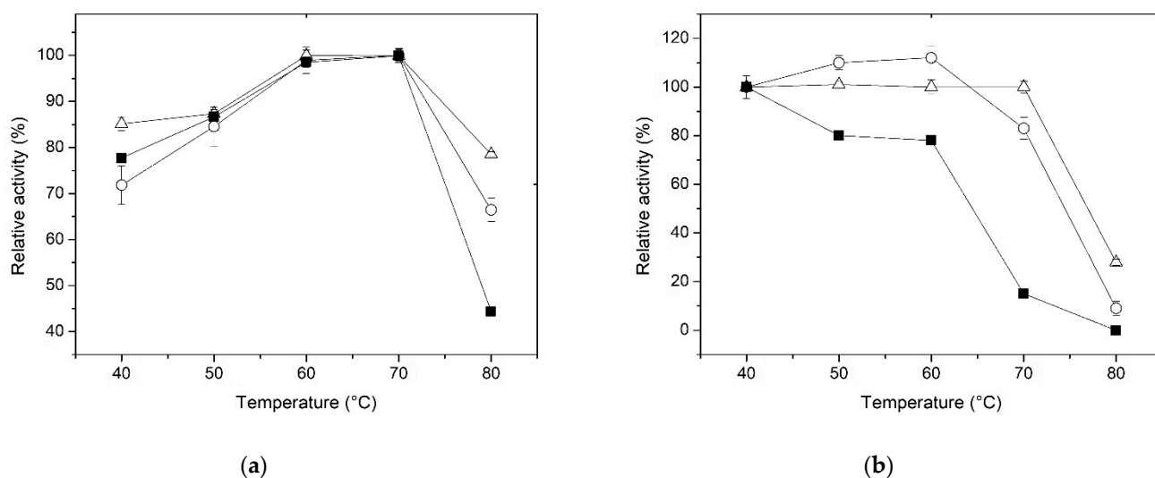
Figure 3. Effect of temperature on the \beta -xylosidase activity (a) and stability (b) of free XynB2 Y509E (■), XynB2 Y509E immobilized by entrapment on chitosan spheres (○), and XynB2 Y509E immobilized on glutaraldehyde-activated chitosan spheres (Δ).
