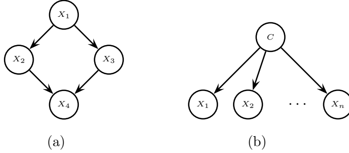
Figure 1. An example of a BN model (a), and the structure of the NB model classifier (b).
