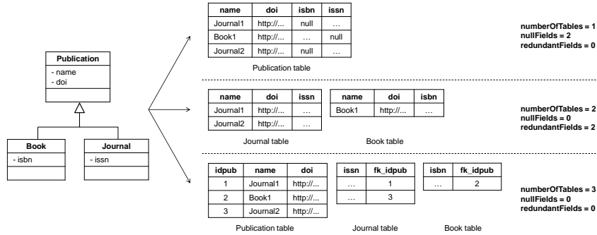
Fig. 1. An example of domain-dependent properties
