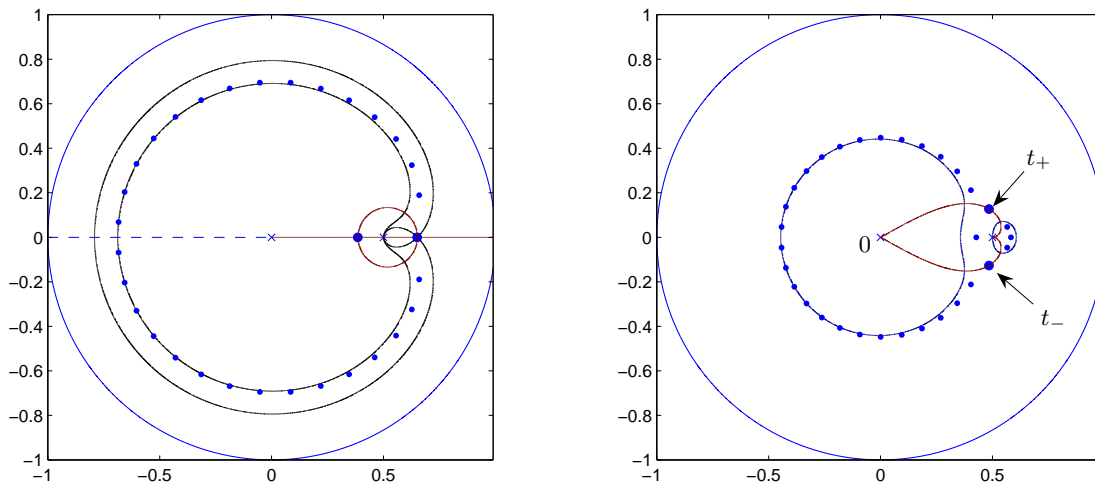
FIG. 2.3. Left: zeros of \Phi_n for w given in (2.30) with \rho = 1/2 and n = 30 , along with the level curves \operatorname{Re}(\Psi_n(z) - \Psi_n(t_+)) = 0 , \operatorname{Re}(\Psi_n(z) - \Psi_n(t_+)) = \frac{1}{n} \log \left( \frac{1}{2\sqrt{\pi}} \frac{\rho^{3/4}}{n^{3/4}} \right) and \operatorname{Im}(\Psi_n(z) - \Psi_n(t_+)) = 0 . Right: the same, but for the weight 1/w . Observe that the level curve (2.32) has now two components.
