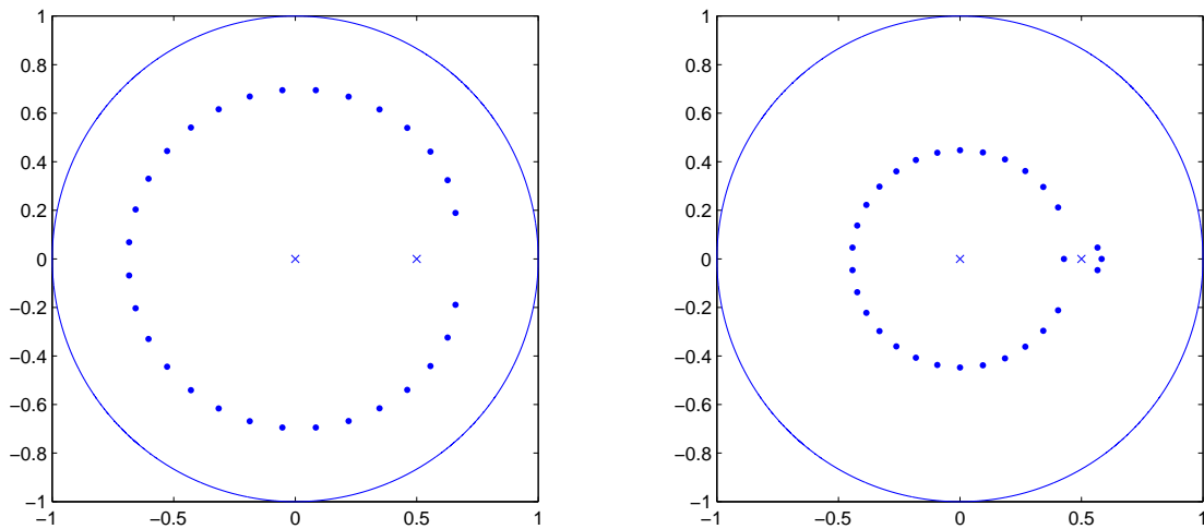
FIG. 2.2. Zeros of \Phi_{30} for weights w (left) and 1/w (right), with w given in (2.30) and \rho = 1/2 .
