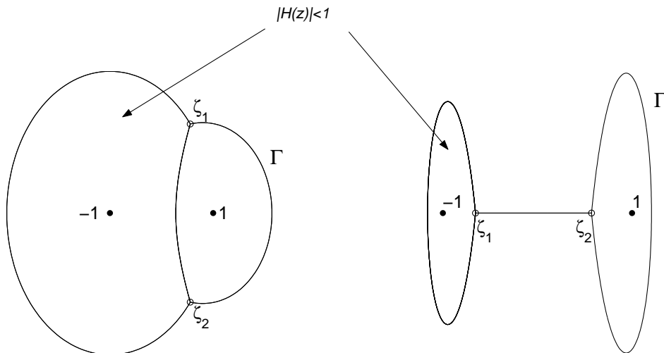
Figure 7: Regions where |H(z)| < 1 for cases C.2 (left) and C.3.
