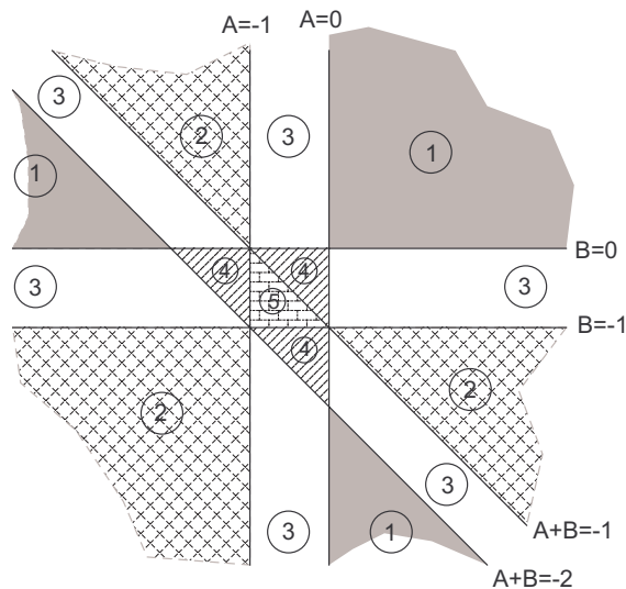
Figure 1: The five different cases in the classification of Jacobi polynomials with varying parameters according to [24].
