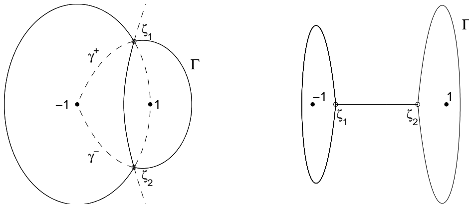
Figure 2: Typical structure of the set \mathcal{N} for cases C.2 (left) and C.3. Dashed lines on the left are orthogonal critical trajectories.
