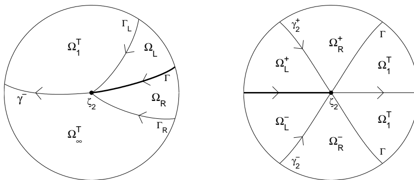
Figure 9: Local analysis for cases C.2 (left) and C.3.
