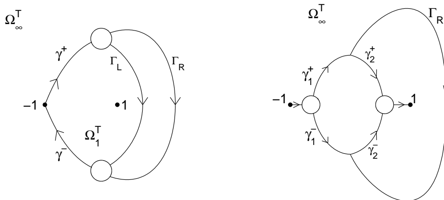
Figure 10: Contours \mathcal{C}^S for S in cases C.2 (left) and C.3.
