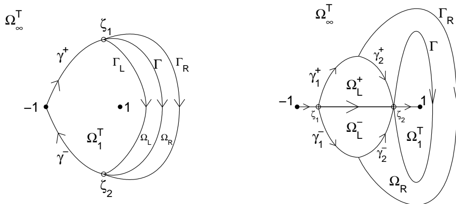
Figure 8: Contours \mathcal{C}^T for T .
