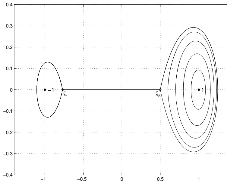
Figure 4: Some trajectories of the quadratic differential (2.3), or equivalently, some level sets \Gamma_r , for the values A = -0.8 and B = 0.5 .
