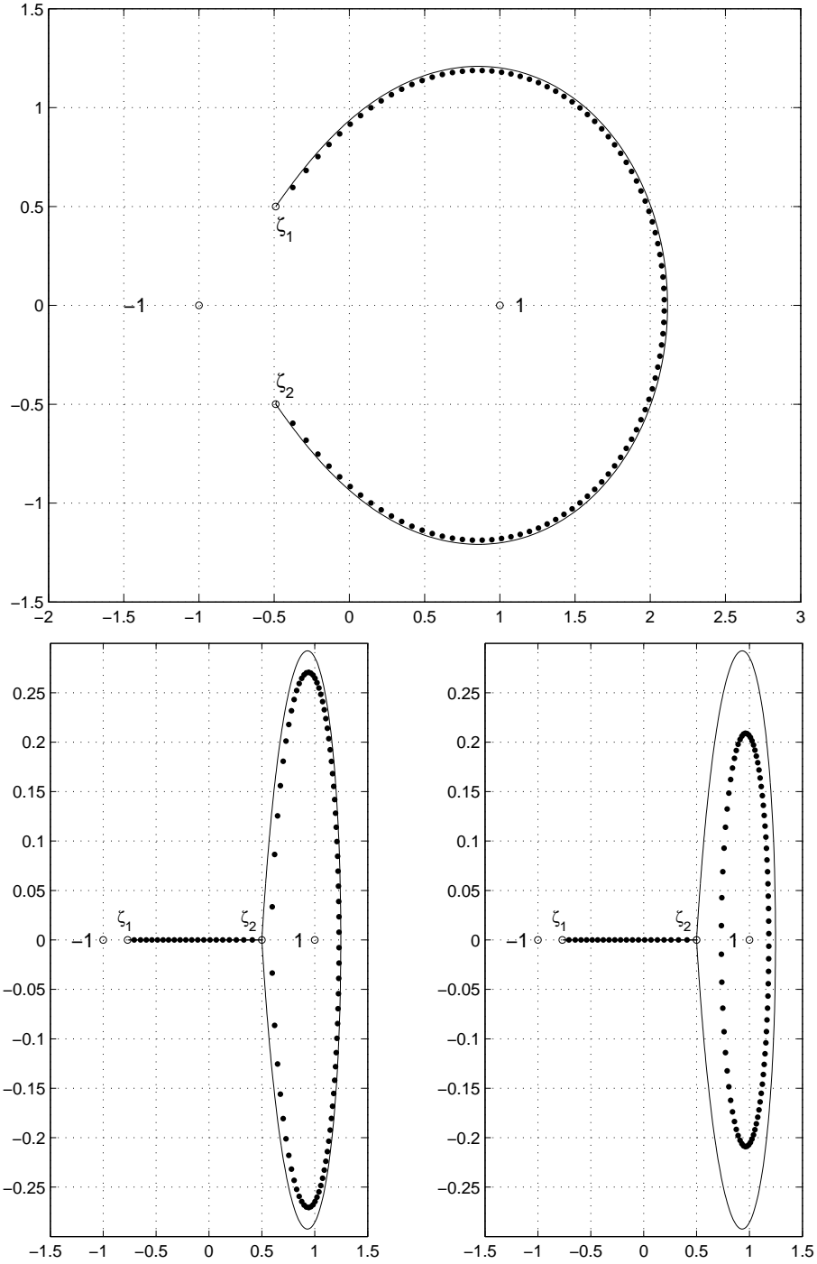
Figure 5: Up, case C.2: zeros of P_{100}^{(-110-10^{-5}, 50-10^{-5})} , along with the curve \Gamma , corresponding to A = -1.1 and B = 0.5 . Down, case C.3: zeros of P_{100}^{(-80-10^{-5}, 50-10^{-5})} (left) and P_{100}^{(-80-10^{-15}, 50-10^{-5})} (right), along with the set \Sigma , corresponding to A = -0.8 and B = 0.5 .
