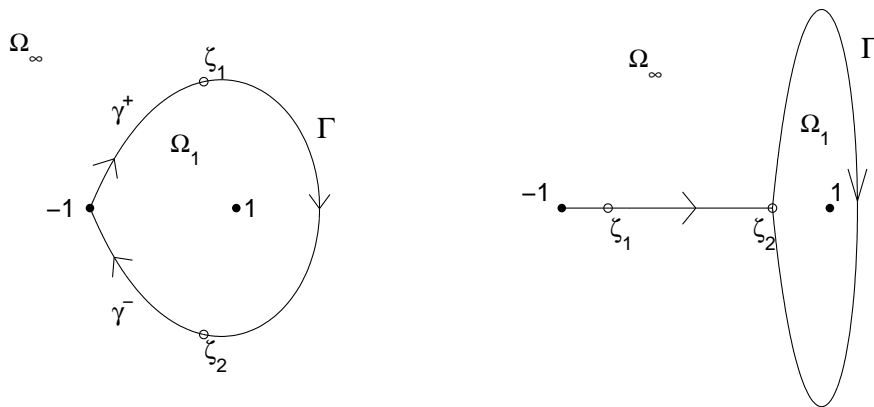
Figure 6: Contours \mathcal{C} for the Riemann-Hilbert problem for Y ; cases C.2 (left) and C.3.
