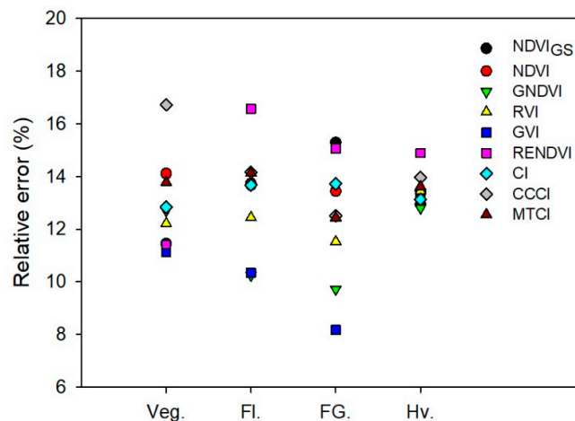
Figure 3. Relative error of linear relationships between observed integrated Nitrogen Nutrition Index (NNI i ) values and predicted NNI i for each vegetation index at different phenological stages, for validation data ( n = 20 ). Veg: Vegetative stage; Fl: Flowering stage; FG: Early fruit growth stage; Hv: Harvest stage. Abbreviations for vegetation indices are in Table 2.
