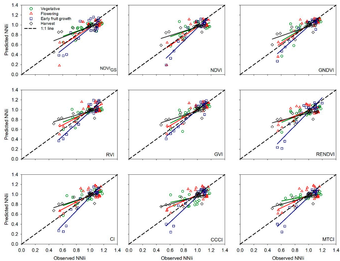
Figure 2. Relationships between observed integrated Nitrogen Nutrition Index (NNII) and predicted NNII for the four phenological stages, for validation data ( n = 20 ). Circle: Vegetative; Triangle: Flowering; Square: Early fruit growth; and Diamond: Harvest stage. Panel (a) shows NDVI measured with GreenSeeker sensor and the other panels (b–i) show indices calculated with Crop Circle sensor. Dotted line represents the 1:1 line. Results of regression are in Table 4. Abbreviations for vegetation indices are in Table 2.
